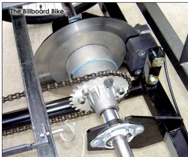
Braking is provided by a revolutionary hydraulic 8-3/4" rear disk brake and supported by a front V brake. A rear differential allows for independent wheel speeds and better maneuverability.
